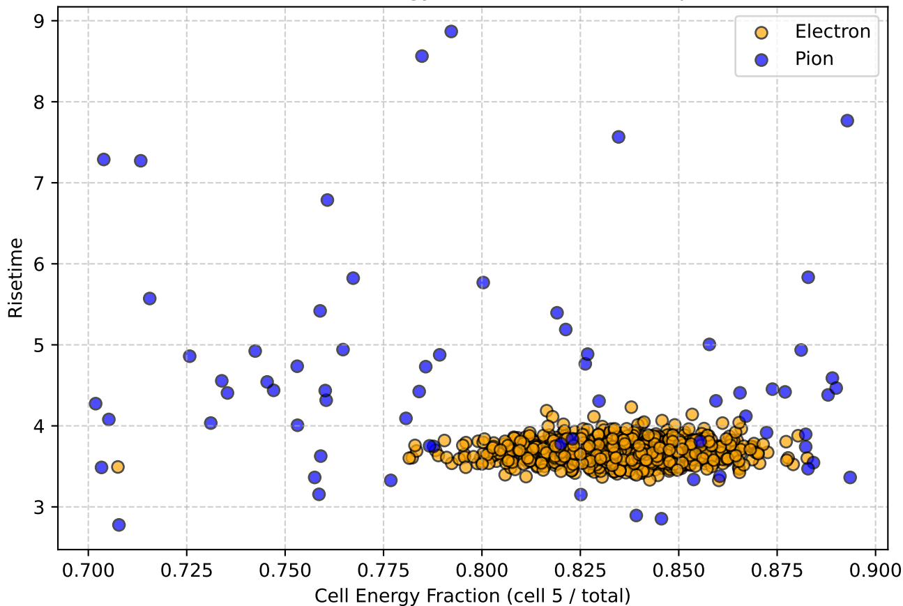
Risetime vs Cell Energy Fraction for 10.0GeV particles
